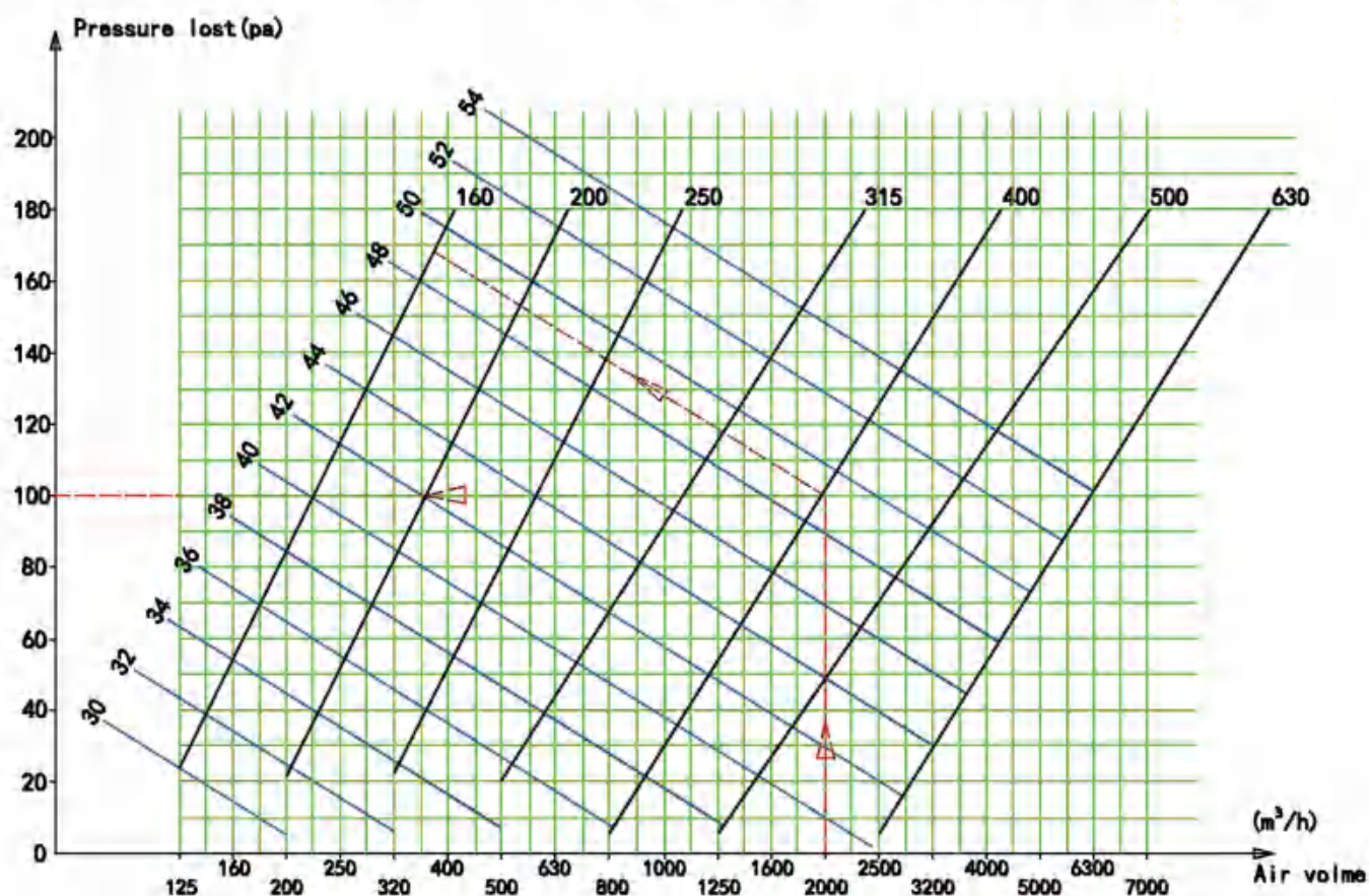
Curve of air volume ,pressure lost and noise for JD-VA Series( V_x=0.5\text{m/s} )
